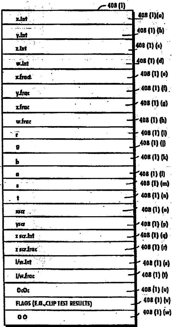
EXAMPLE VERTEX DATA STRUCTURE
